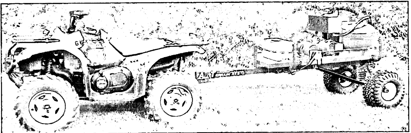
'ATR-2' Folding Frame Res-Q Trailer shown with ATR - CAFS-21 skid option.
